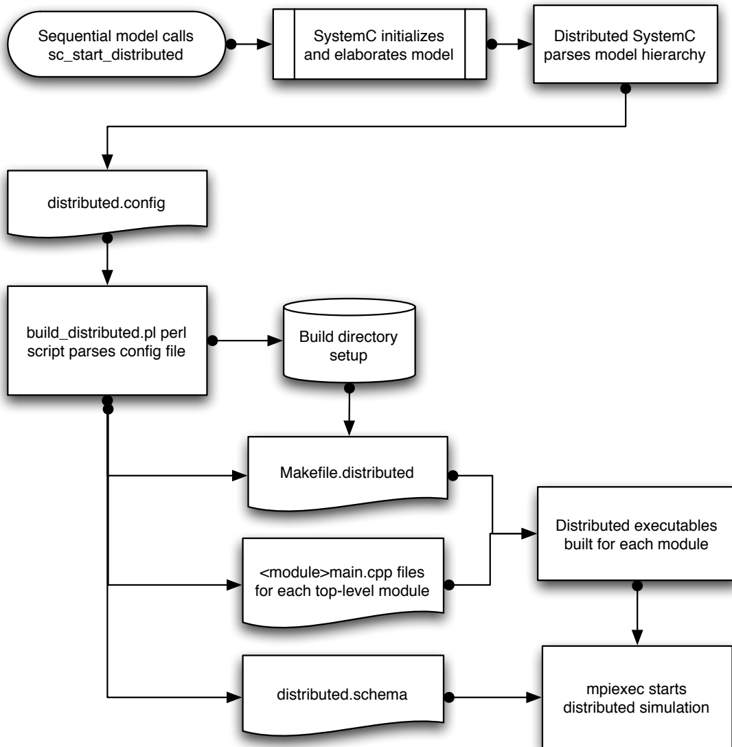
Figure 4.4: Automated distribution process and output files
