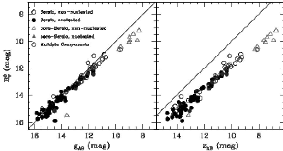
FIG. 16.— Comparison of the g and z -band total magnitudes, corrected for extinction, derived by integrating to infinity the best fitting surface brightness profiles, compared to the B_{g0}^0 magnitudes from the RC3. The diagonal line shows a one-to-one correspondence. Galaxies with multiple morphological components, for which the model fits are not always satisfactory, are plotted in blue.
