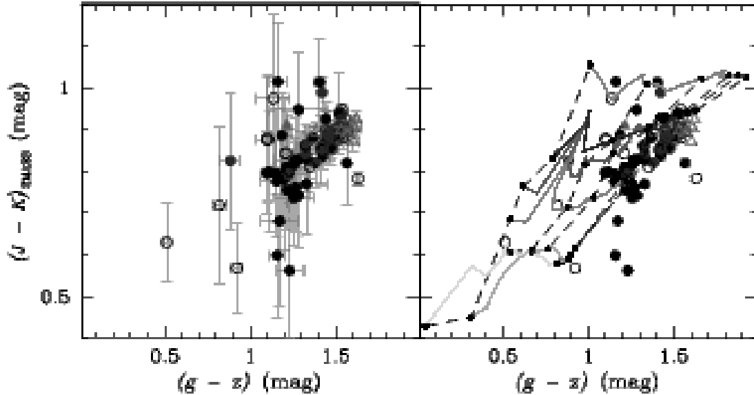
FIG. 25.— g-z vs J-K color-color diagrams. J and K -band magnitudes are from the 2MASS database. Galaxies are coded as in Figure 24, as are the stellar population synthesis models. All magnitudes have been extinction corrected.
