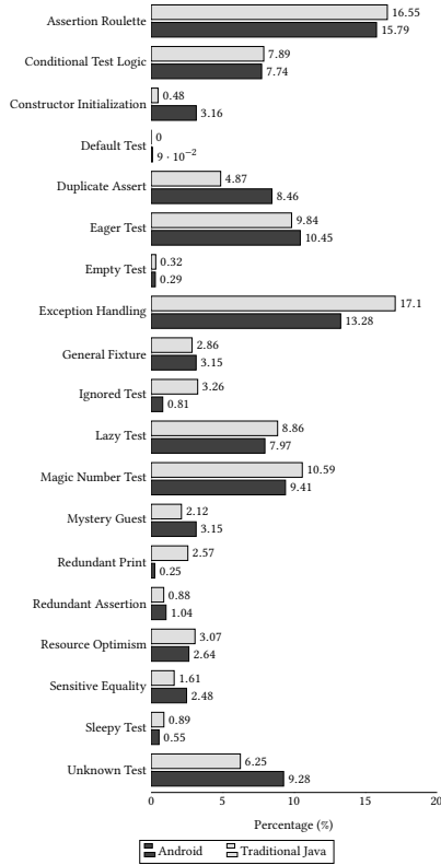
Figure 2: The distribution of the different test smell types in traditional Java and Android applications
