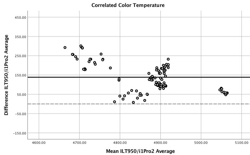
Figure 1. Bland-Altman Plot comparing CCT readings from ILT950 with the average of the X-Rite i1Pro 2 across the range of viewing booths. The bold solid horizontal line indicates the mean difference, the dashed line indicates zero.
