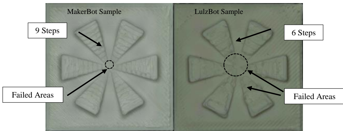
Figure.7. Convergent slanted ray GETTs divulges FDM printers' z-direction addressability through the number of steps on the slanted plane for a given height.
