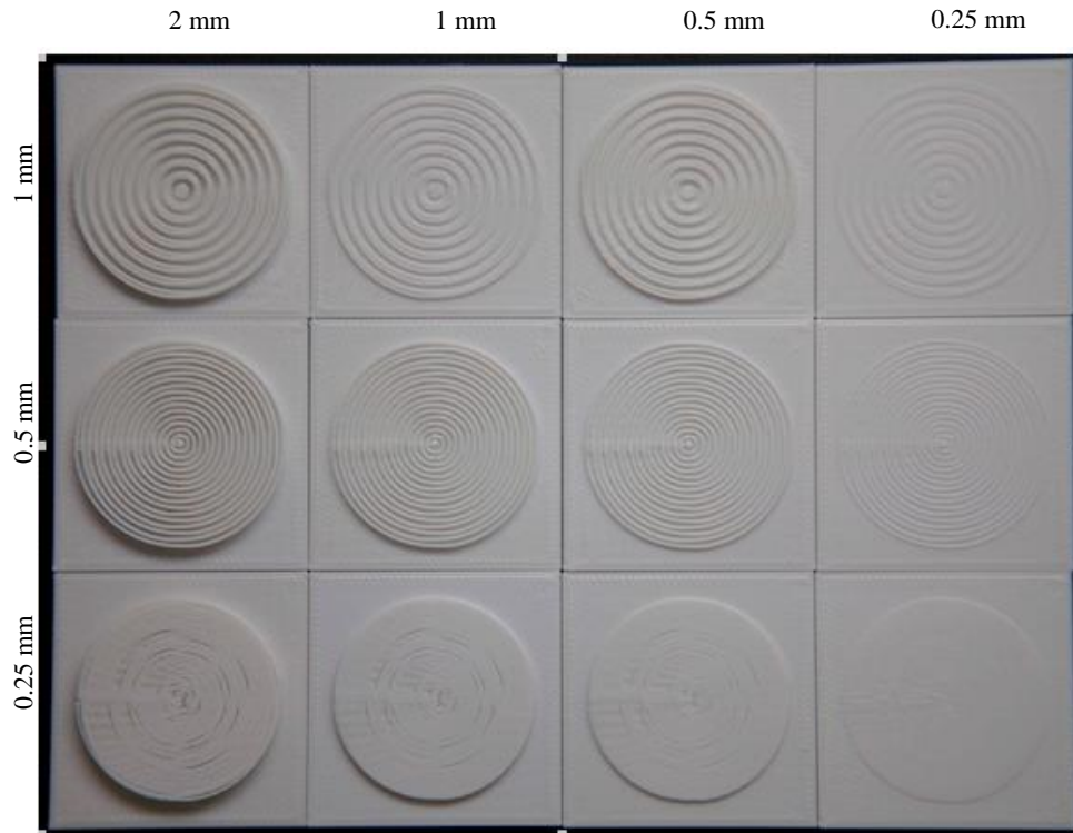
Figure.9. Height and frequency resolution concentric circle GETTs to detect dimensional failures and deviations.
