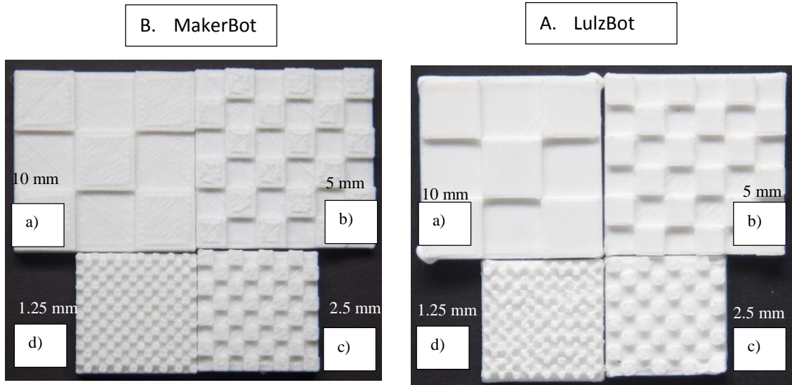
Figure.5. A sequence of decreasing sizes of checkerboard patterns shows resolution limitation difference of two FDM devices to produce squares. The device that produced the left group of GETTs, MakerBot, loses its ability at about 1.25 mm checker size. In contrast, the device that produced the right group of GETTs, LulzBot, fails at about 2.5 mm checker size.
