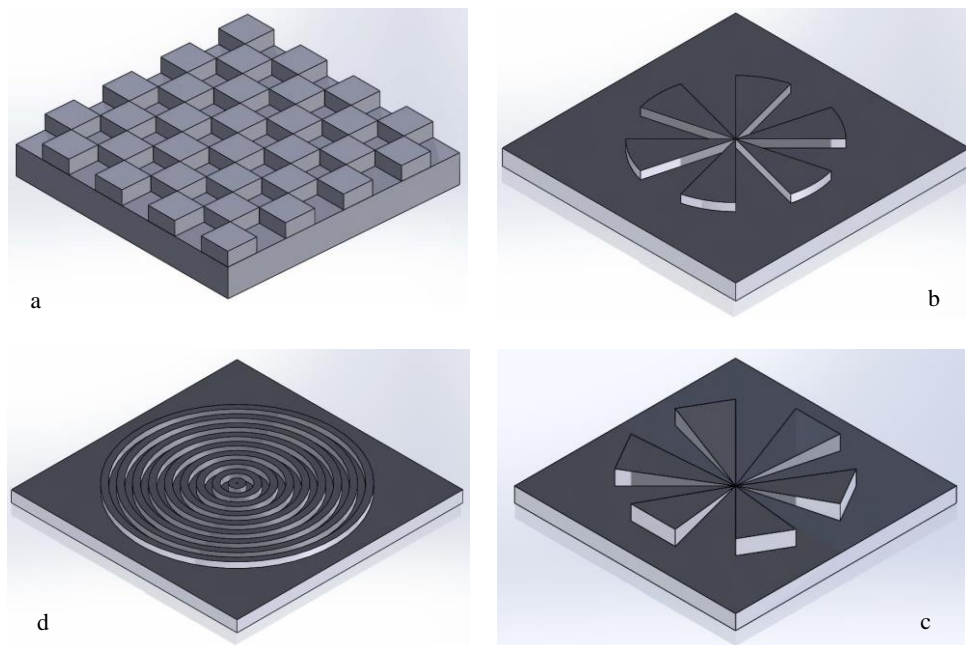
Figure.4. Perspective view of checkerboard (a), flat ray (b), slanted ray (c), and concentric circle (d) GETTs respectively.
