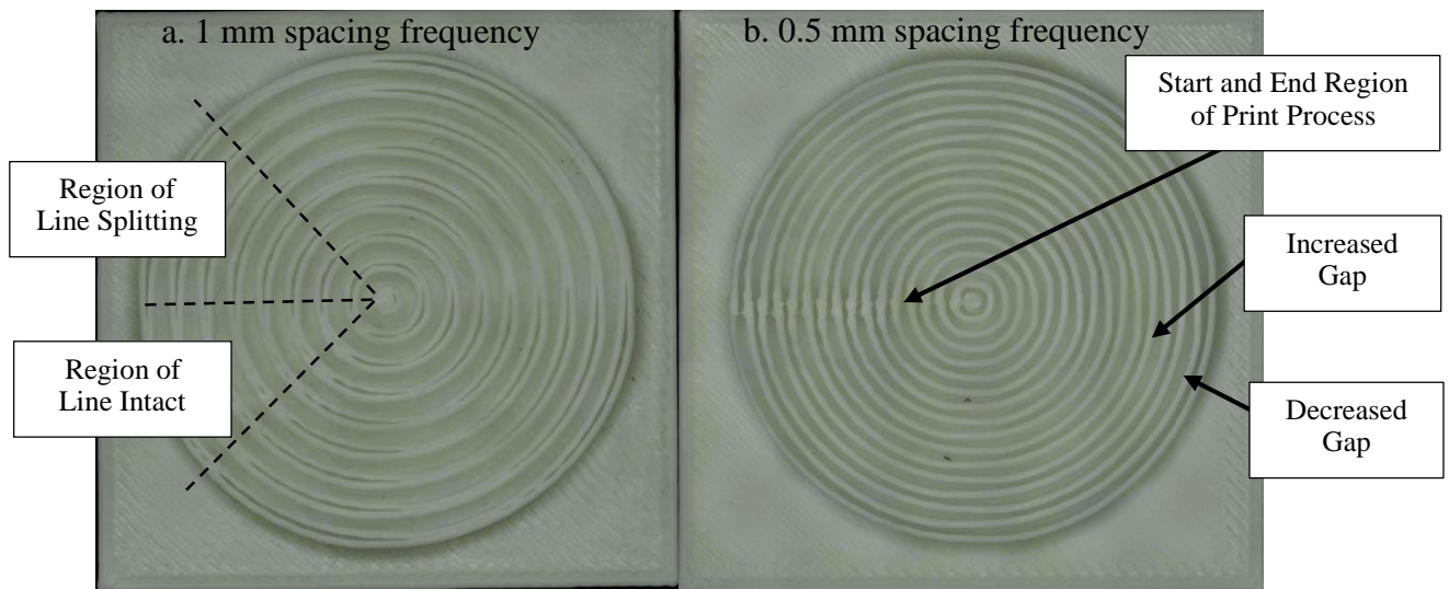
Figure.8. Concentric circle targets to illustrate defects of FDM printing: line splitting, deviations in print paths, and visible joining of start and end points.
