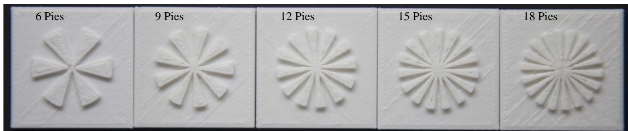
Figure.6. A sequence of increasing number of pies in ray GETTs. The resulted center rings mark the areas that the printer has failed to print. These areas can be used to calculate the resolvable line width.
