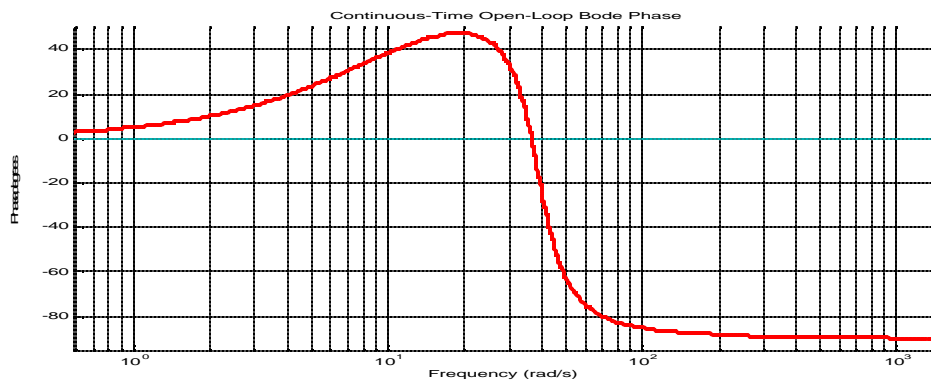
Figure 4. Bode phase plot of the system.
