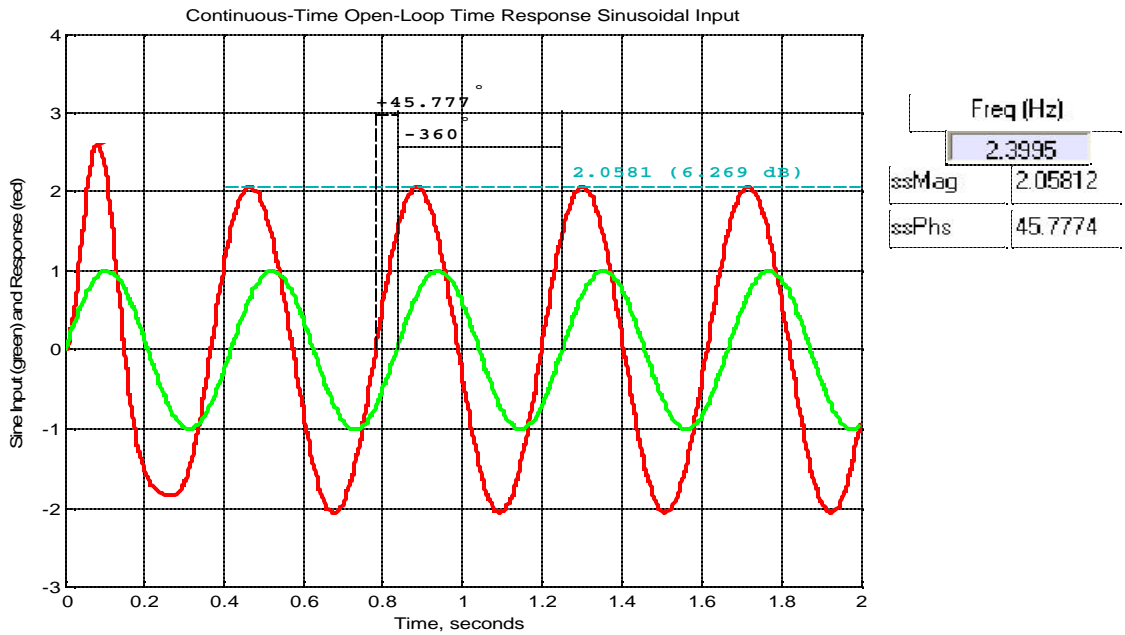
Figure 2. Time-domain plot of the sinusoidal response to a 2.4 Hz sinusoid.
