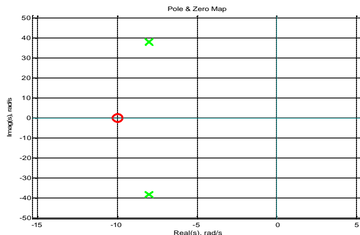
Figure 1. Pole/zero map showing the model of a linear system (not including gain).
