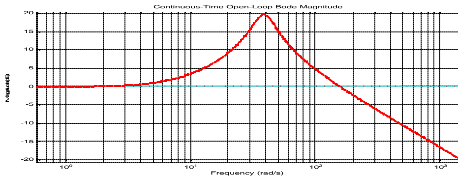
Figure 3. Bode magnitude plot of the system.
