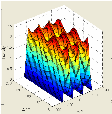
Fig. 4.3 3-D image in resist.
