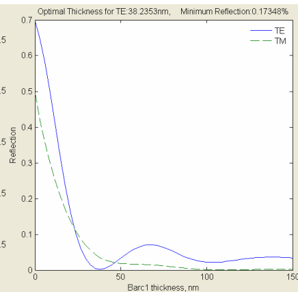
Fig.4.6.1 Substrate (BARC) reflection.
