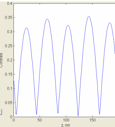
Fig. 4.4 Image contrast in resist.
