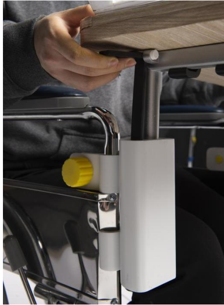
Figure 11. Table handle and support structure
