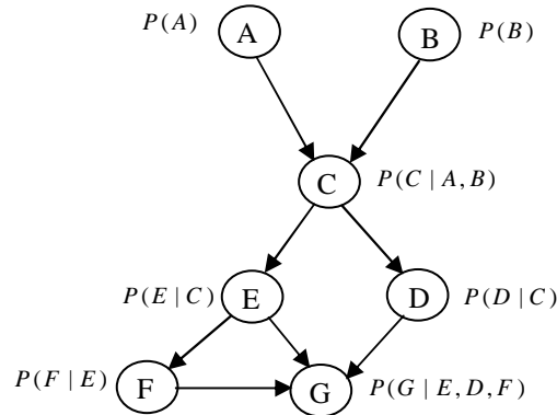
Fig. 1. A directed acyclic graph (DAG). The probabilities to specify are shown.
