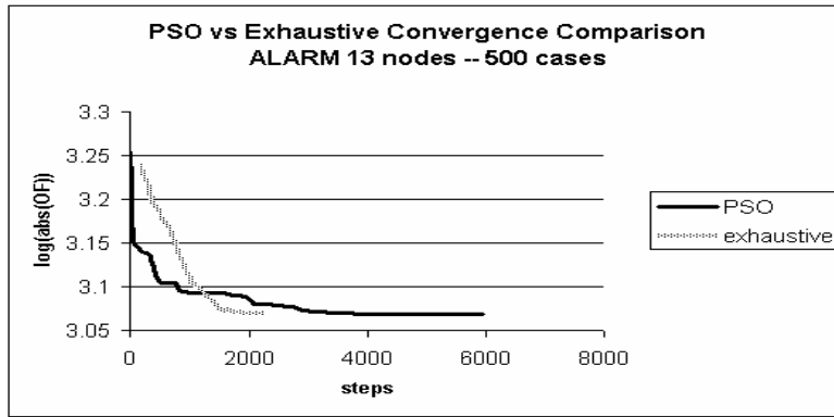
Fig. 3. Complexity comparison, PSO vs. Exhaustive Heuristic
