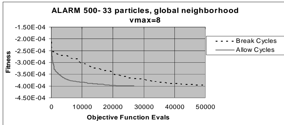
Fig. 4. Allowing cycles versus breaking cycles in PSO.
