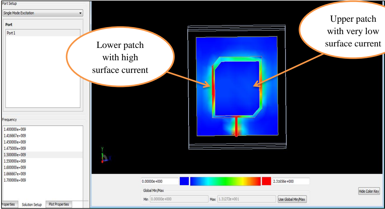
Fig.80 Surface Current of the electromagnetically coupled two patches
