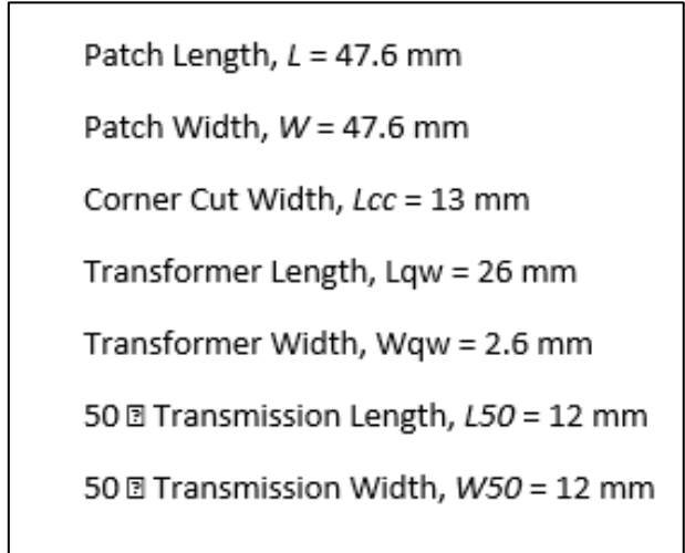
Fig.38 Antenna design parameter of the work [16]
