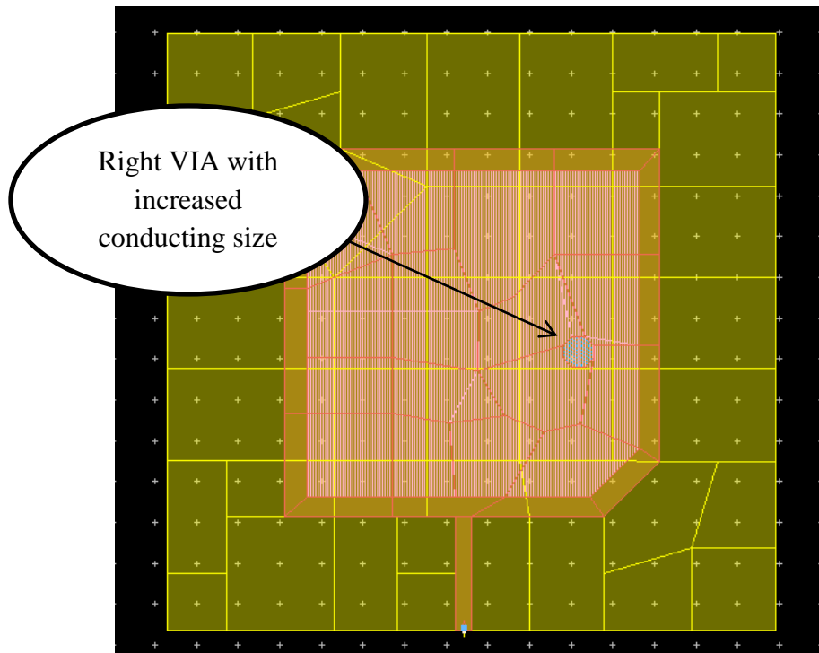
Fig.85 Antenna with Right VIA, and increased VIA conductor size
