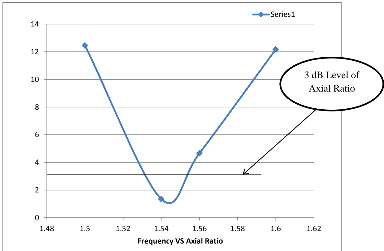
Fig.75 Axial Ratio of the simple antenna
