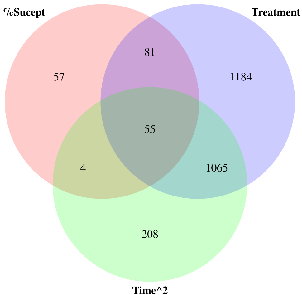
Figure 16: Venn diagram showing overlapping significant genes by model
