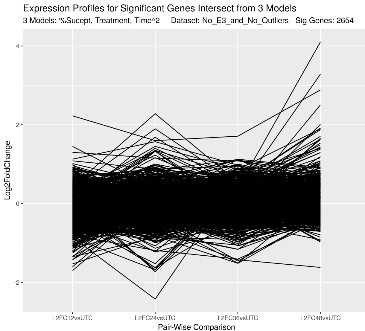
Figure 17: Vitis vinifera Expression Profiles for Significant Genes
