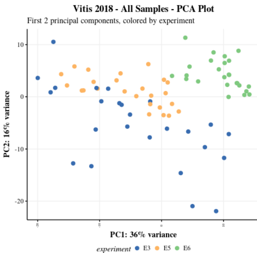
Figure 15: Vitis vinifera PCA for all samples
