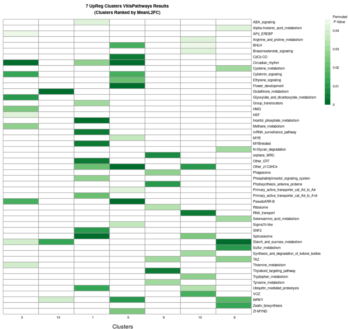
Figure 32: Up-regulated Pathways for Vitis vinifera Clusters
