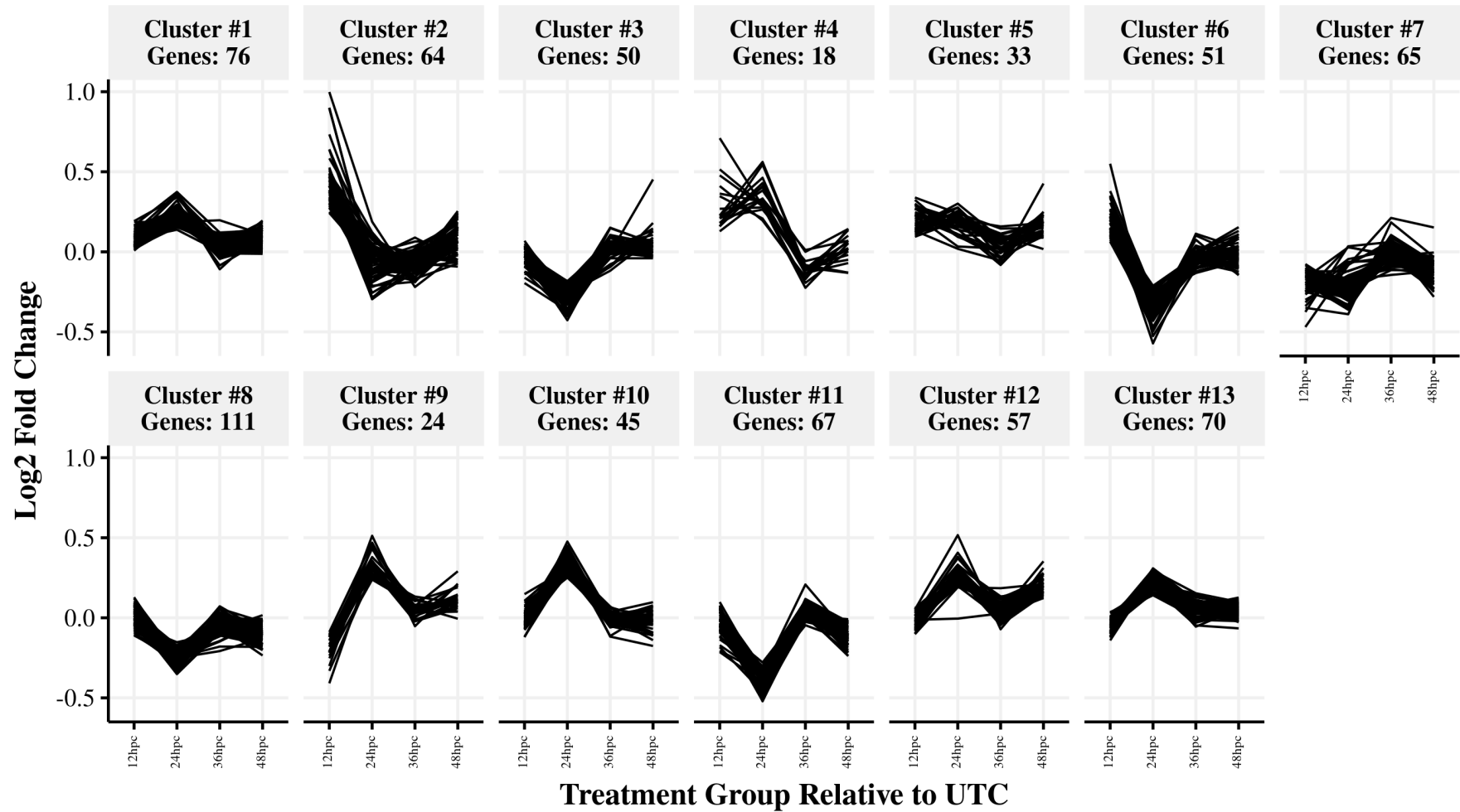
Figure 23: Arabidopsis thaliana Gene Expression Clusters
