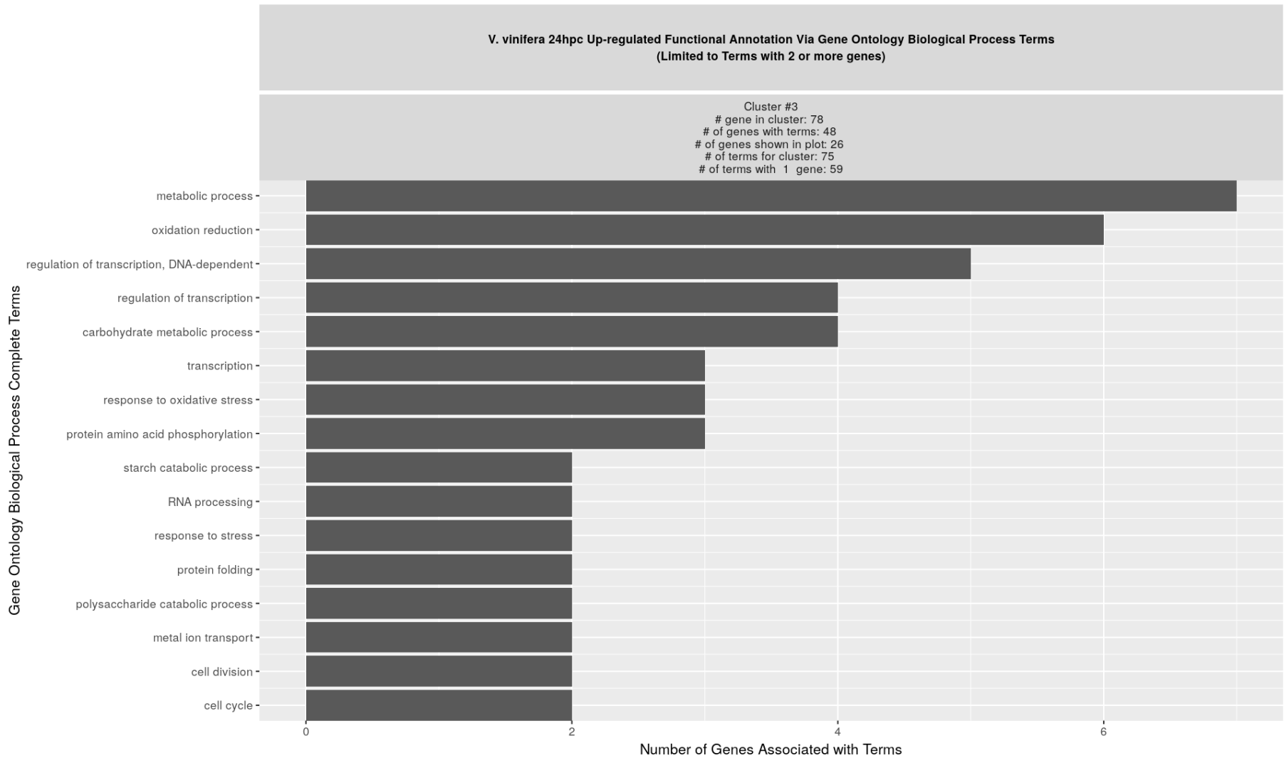
Figure 25: Vitis vinifera - 24hpc up-regulated (cluster #3) biological process GO terms
