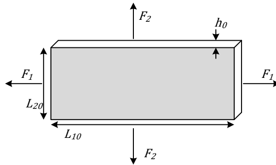
Figure 2.4. Stress-force relationship on a simple 3D object, where F_1, F_2 represent force in the x,y direction, respectively. L_{10}, L_{20} represent the initial unstressed length in the x,y direction, and h_0 represents the initial unstressed thickness.
