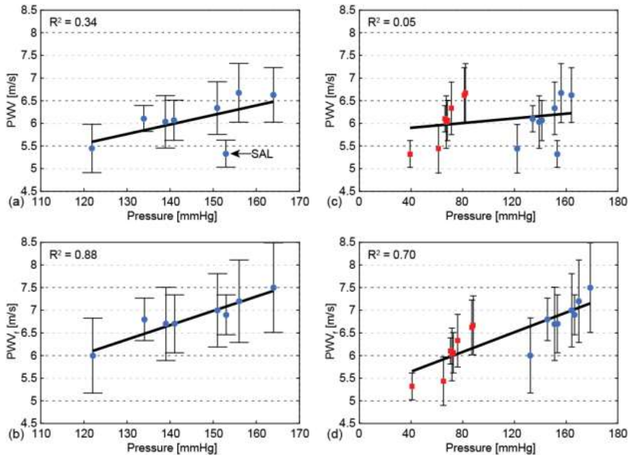
Figure 6.4. PWV_i measured at the finger improves blood pressure prediction. Error bars represent the standard deviation for PWV calculated from the referenced TT measurement [15] and uncertainty in measures required for calculation of flow velocity. For all figures, the systolic pressure is represented by a circle, and the diastolic pressure is represented by a square. The left side includes SBP only; the right side includes both pressures (SBP and DBP). a) PWV uncorrected for flow across measured SBP. Salbutamol (SAL) was the farthest of any other measure from the trend line. b) PWV corrected for flow velocity improves the correlation with SBP alone. c) The lowest correlation was observed with PWV uncorrected for flow across measured pressures. d) PWV corrected for flow velocity improves the overall correlation across all pressures. Analysis of diastolic pressure versus PWV (data not shown) produced R^2 = 0.85 .
